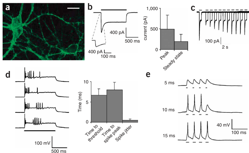
Figure 1 ChR2 enables light-driven neuron spiking. (a) Hippocampal neurons expressing ChR2-YFP (scale bar 30 \mu\text{m} ). (b) Left, inward current in voltage-clamped neuron evoked by 1 s of GFP-wavelength light (indicated by black bar); right, population data (right; mean \pm s.d. plotted throughout; n = 18 ). Inset, expanded initial phase of the current transient. (c) Ten overlaid current traces recorded from a hippocampal neuron illuminated with pairs of 0.5-s light pulses (indicated by gray bars), separated by intervals varying from 1 to 10 s. (d) Voltage traces showing membrane depolarization and spikes in a current-clamped hippocampal neuron (left) evoked by 1-s periods of light (gray bar). Right, properties of the first spike elicited ( n = 10 ): latency to spike threshold, latency to spike peak, and jitter of spike time. (e) Voltage traces in response to brief light pulse series, with light pulses (gray bars) lasting 5 ms (top), 10 ms (middle) or 15 ms (bottom).
